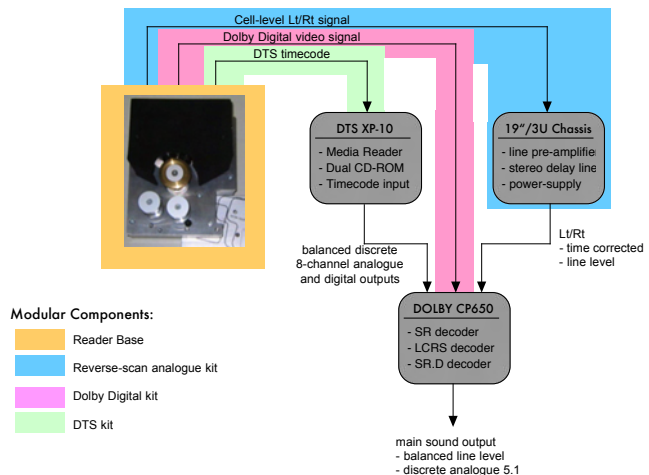
Application Diagram - Fully Decoded Outputs
